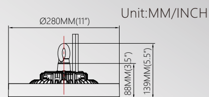
Hanging ring
