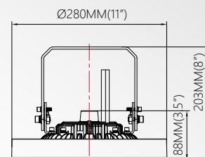
U-Bracket(Options)
